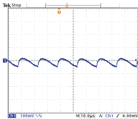
c. Mains input 132 V / 60 Hz (Ch1 = V OUT )
