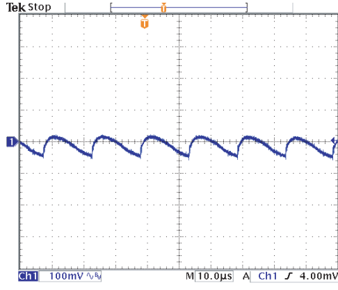
b. Mains input 115 V / 60 Hz (Ch1 = V OUT )
