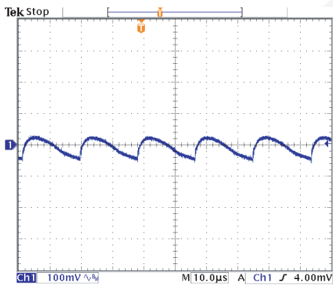
a. Mains input 90 V / 60 Hz (Ch1 = V OUT )
