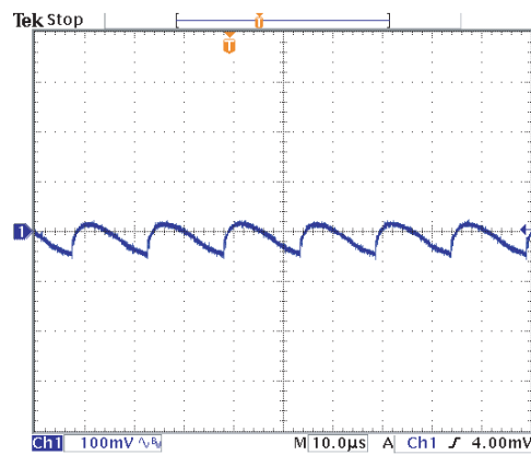
d. Mains input 180 V / 50 Hz (Ch1 = V OUT )
